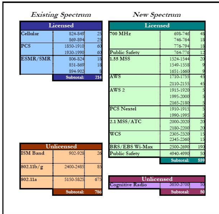
Figure 1: Existing and New Spectrum Bands (2006)
